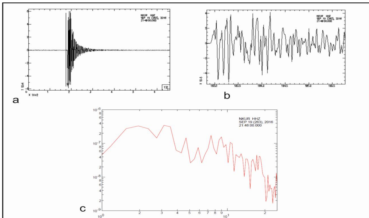
Figure 3: Example of event No. 4 from NKUR station (19/09/2016). The vertical component of the extracted waveform's P-wave's arrival time is shown in (a), the time window employed is shown in (b), and the output logarithmic spectrum is shown in (c).
